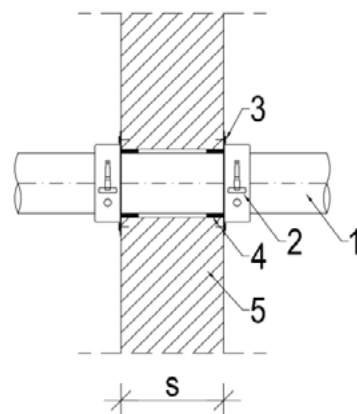
Wall penetration
