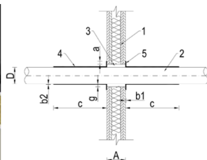
Penetration with mortar filling
