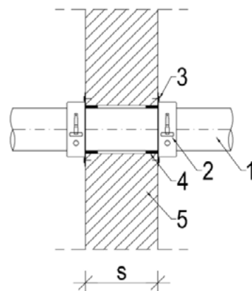
Wall penetration
