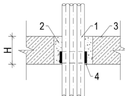
A bundle of pipes in a floor
