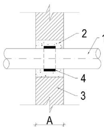
A single pipe in a wall
