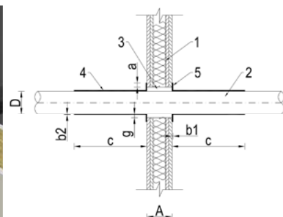
Penetration with mortar filling
