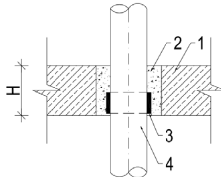
A single pipe in a floor
