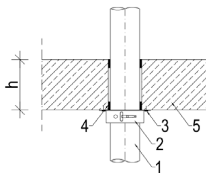
Floor penetration
